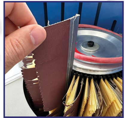
Easy to change paper
