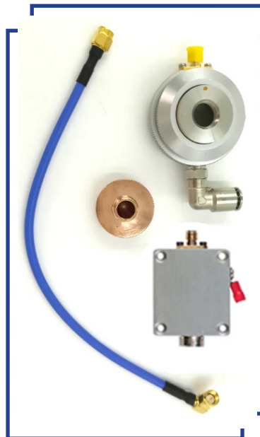
Hybrid Laser Head Signal Filter
