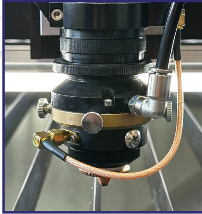
Industrial laser head
