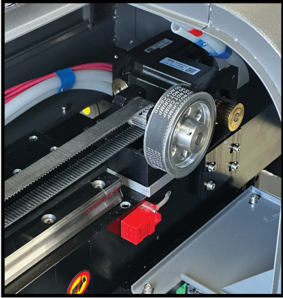
Stepper 86 motor
